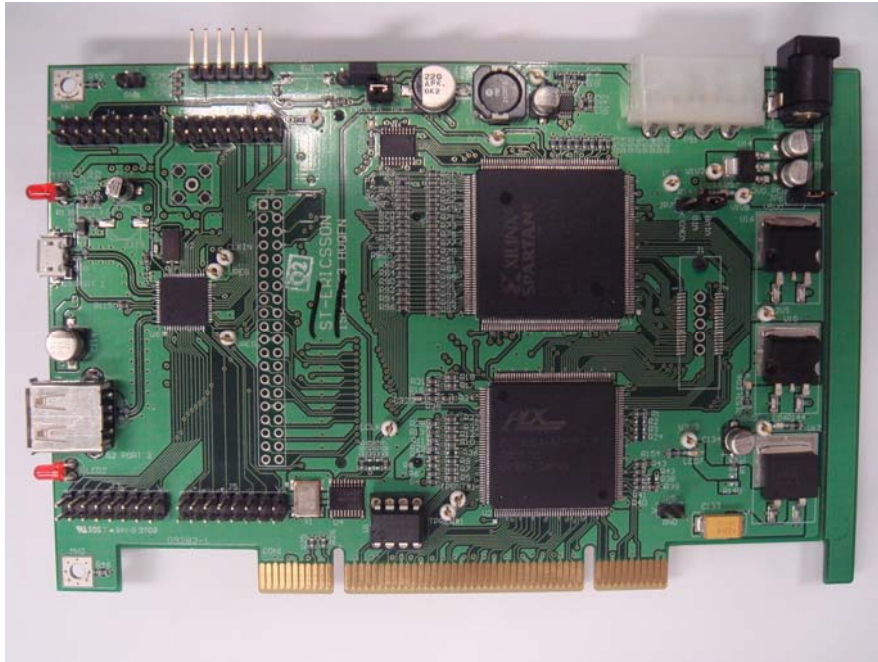
Figure 2 ISP1763A PCI evaluation board—VFQFP
