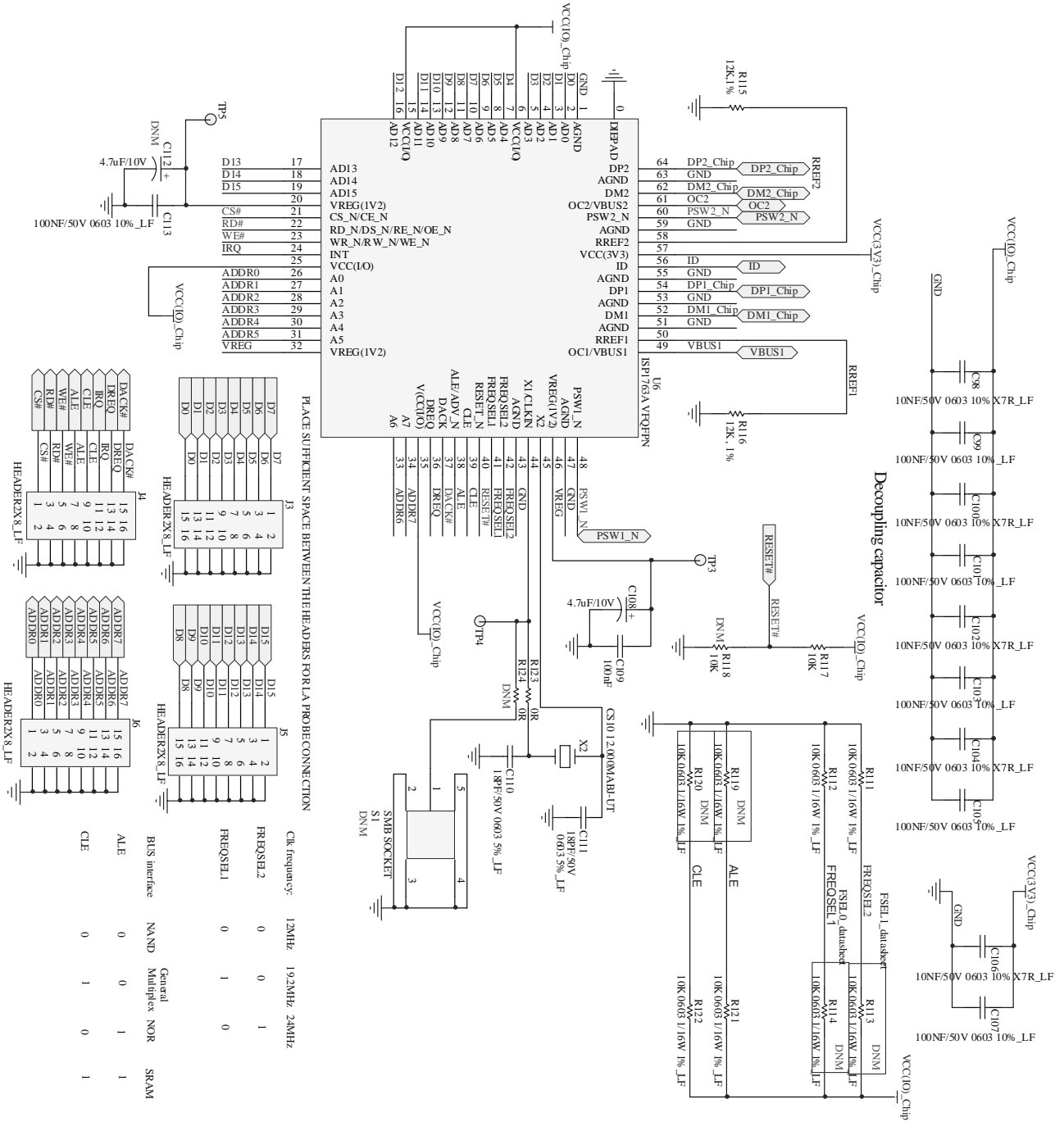
Figure 14 ISP1763A
